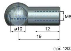
5-2-M8 Kugelpfanne Ball joint housing Coussinet sphérique Cuscinetto sferico Cojinete esférico
