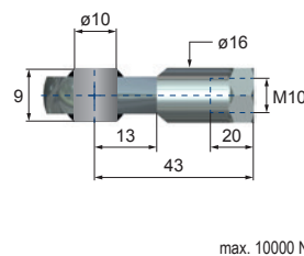
4-M10 Gelenkkopf Spherical end bearing Joint articulé • Forcella snodata Charnela macho articulada
